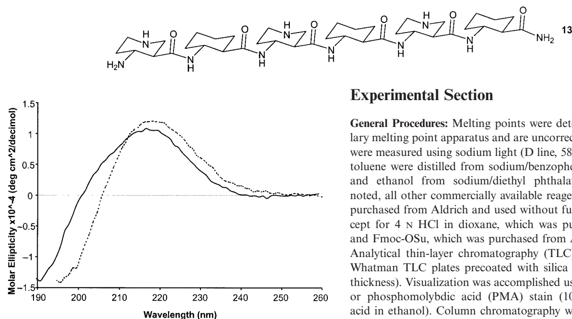
Figure 2. Circular dichroism spectra of hexamer 13 in 10 mM aqueous Tris, pH = 7 (solid line) and in methanol (dashed line)
