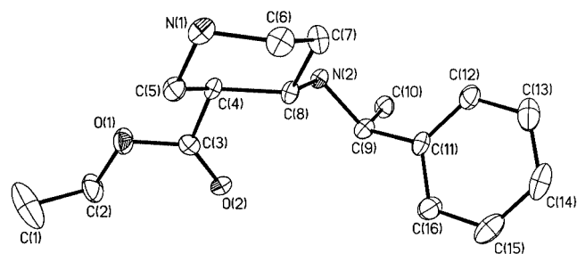
Figure 1. Ball-and-stick representation of the conformation determined crystallographically for 5 in the solid state (H atoms not shown)
